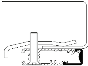
Fig. 5 0.39" Profile mounted using a fixing clamp plate
