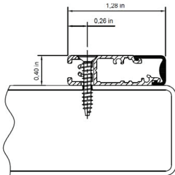
Fig. 4 0.39" Profile fixed with countersunk self-tapping screw
