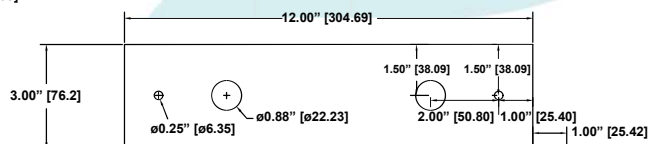
CABINET BACK BOX
